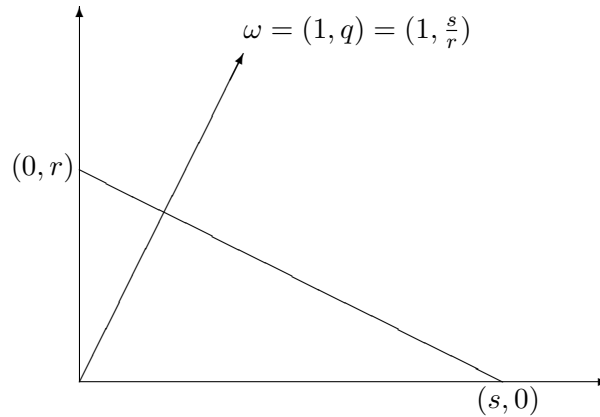
Figure 2.3: (s, 0) and (0, r) on the same line x + qy = s
