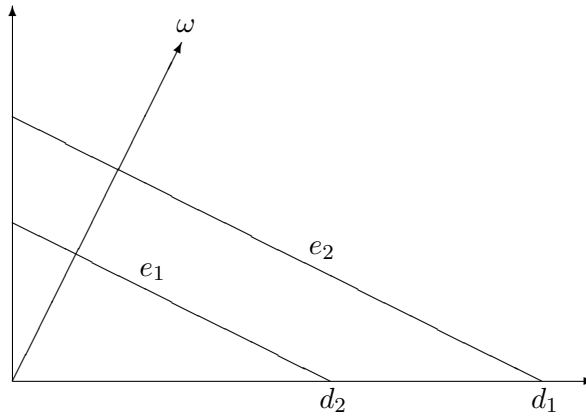
Figure 2.1: \omega = \omega_m = (1, m)
