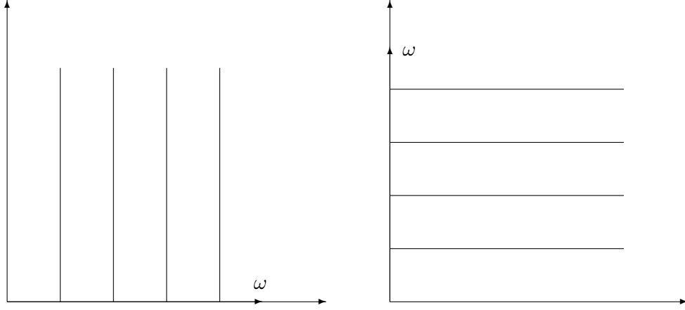
Figure 2.4: 0^+ and \infty^- order
