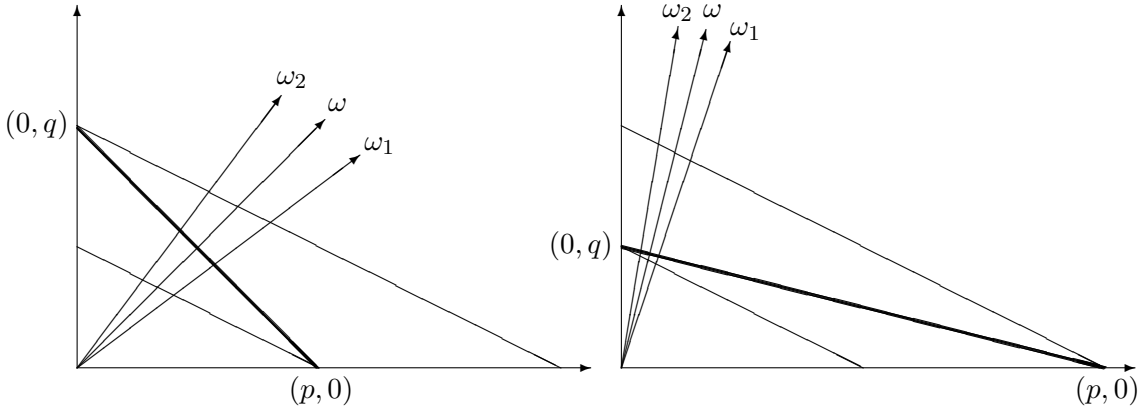
Figure 2.2: \omega_1 = (1, m_1) , \omega_2 = (1, m_2)
